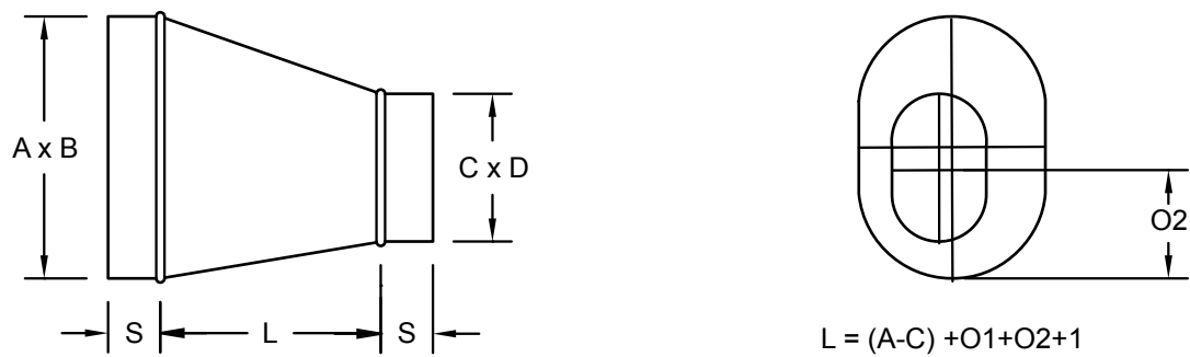
TRANSITION-EASY
