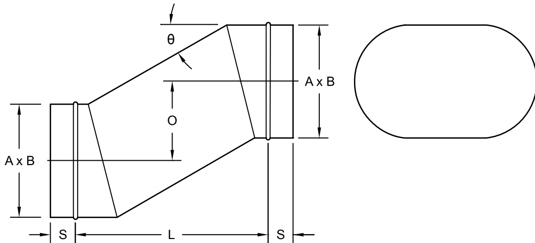
OFFSET EASY
